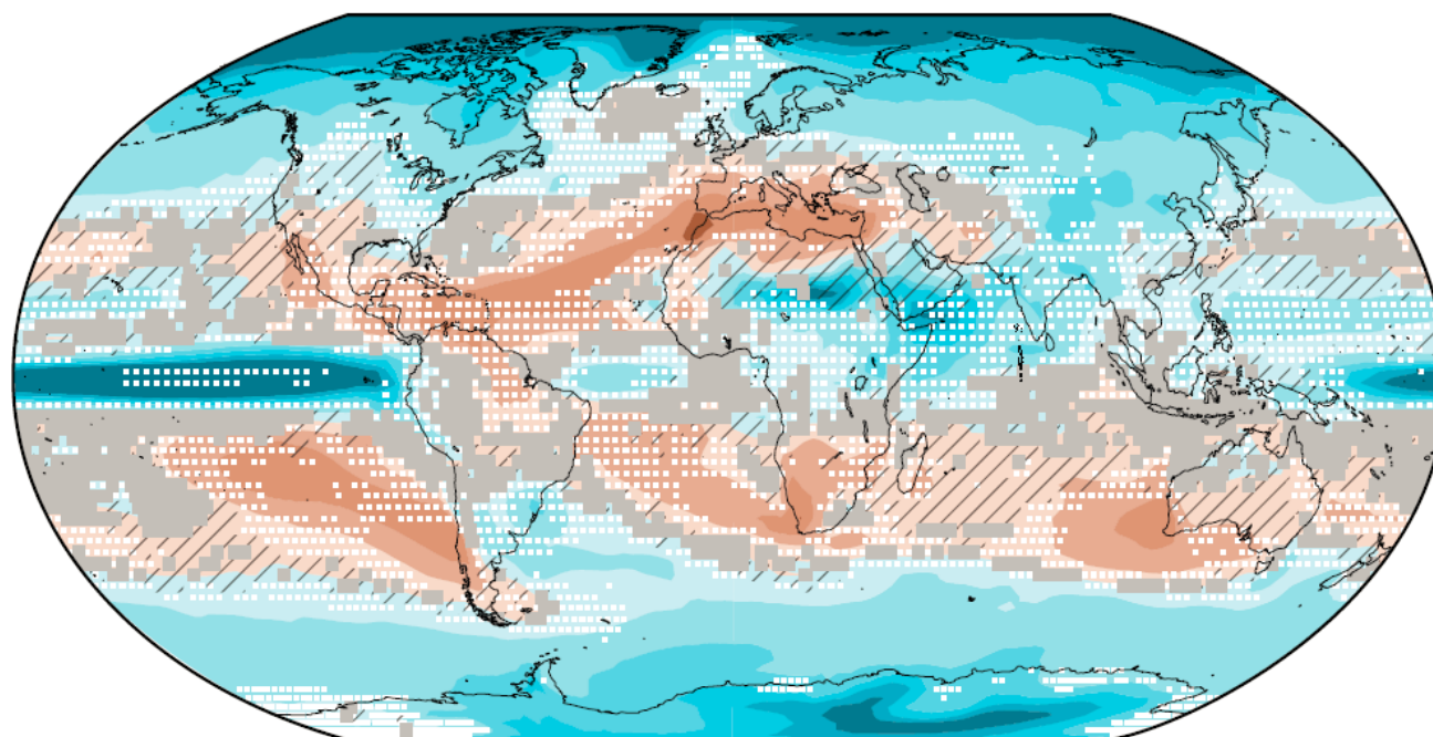
RCP8.5 2081 - 2100
