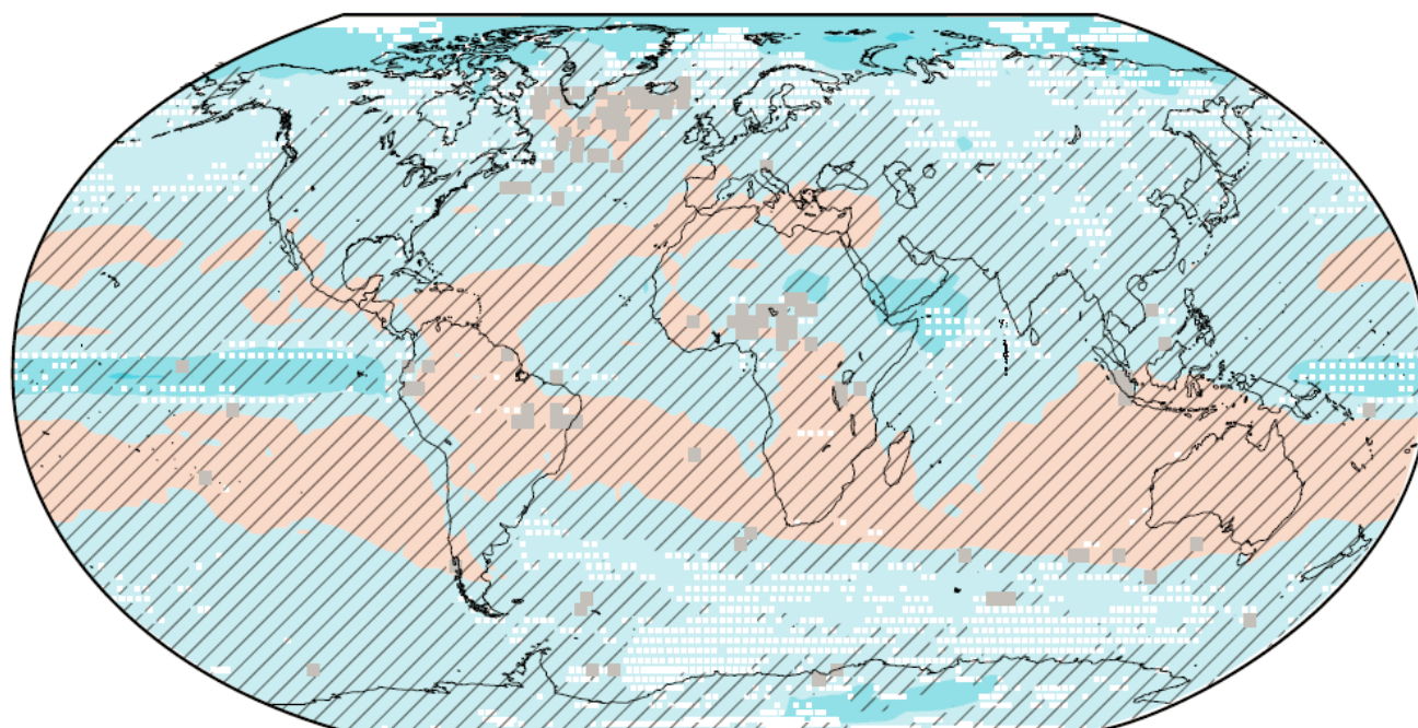
RCP2.6 2081 - 2100
